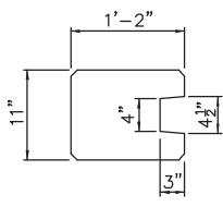
END PILASTER 148 lbs./ft.
