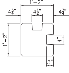
90° PILASTER 183 lbs./ft.
