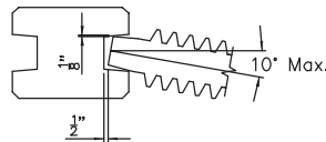
CONSTRUCTION TOLERANCE DIAGRAMS
