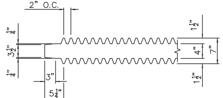
TYPICAL PANEL SECTION
