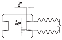
CONSTRUCTION TOLERANCE DIAGRAMS
