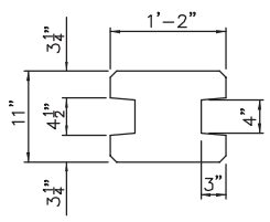
STANDARD PILASTER 136 lbs./ft.
